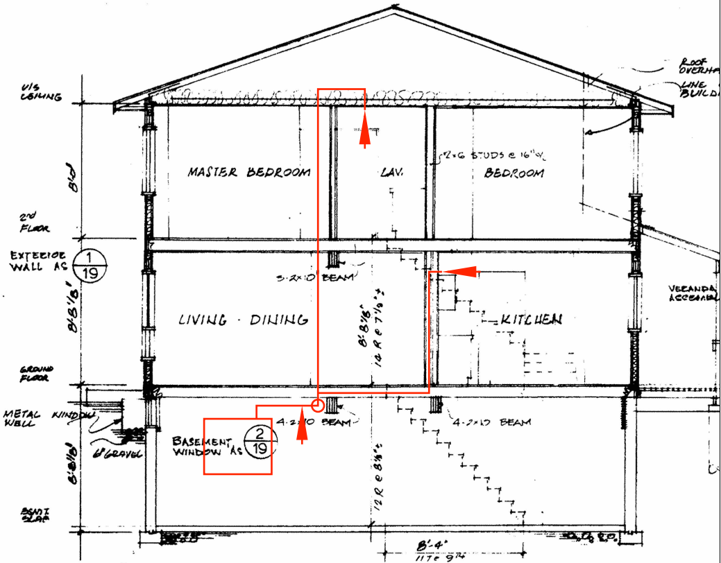
6 Section
