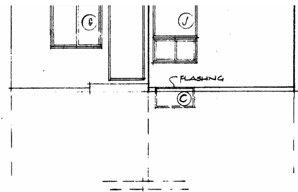
6/9 Patio Elevation
