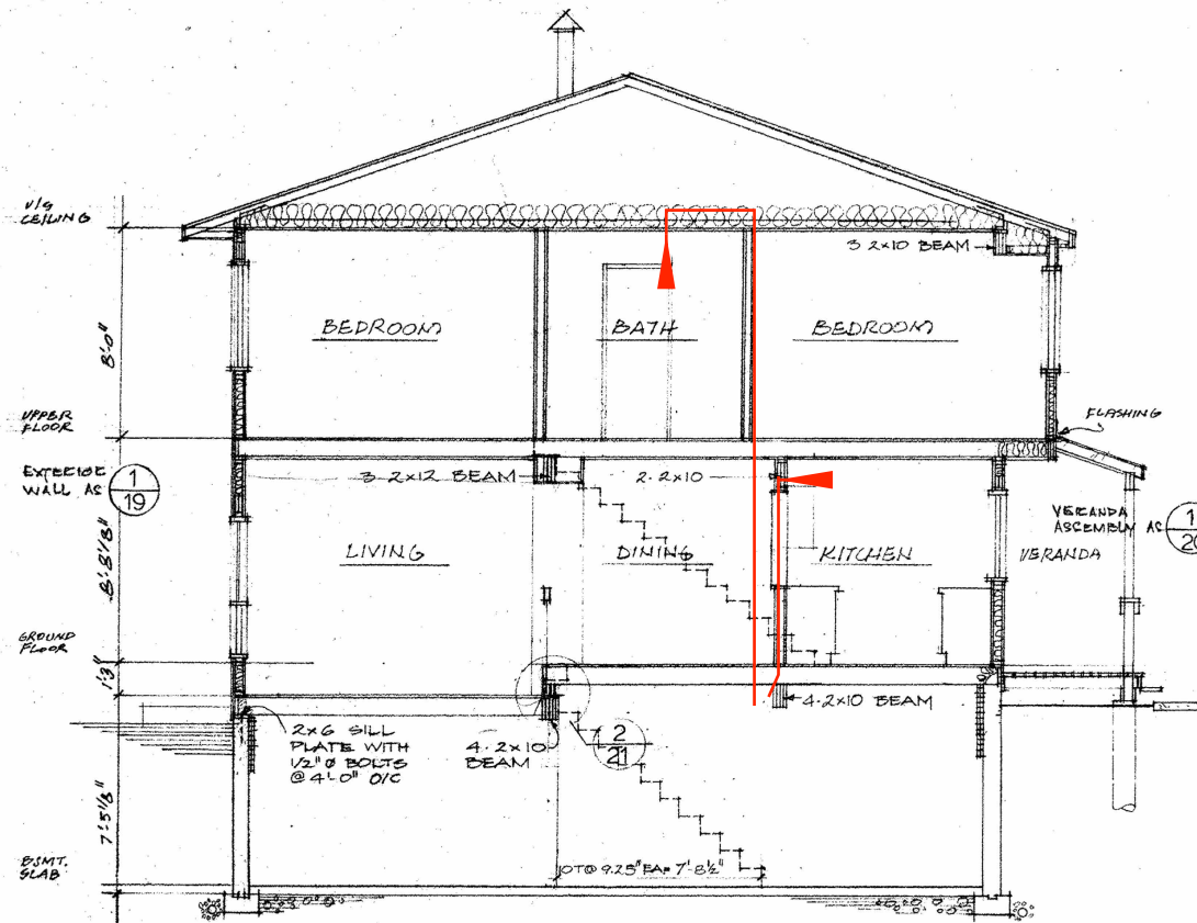
6 Section
