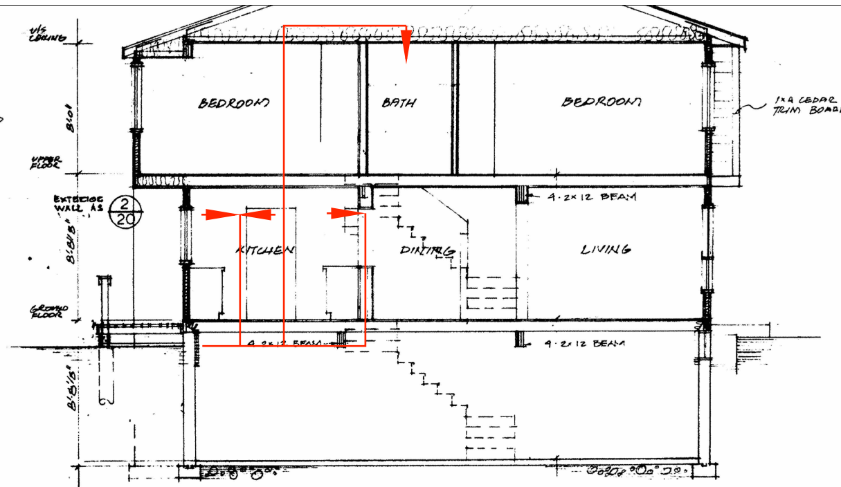
6 Section
