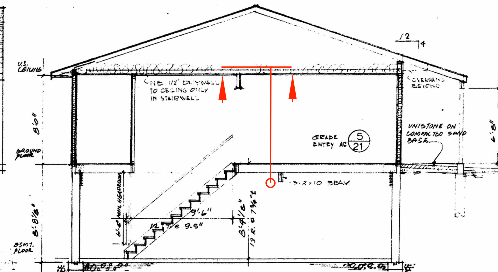
5/8 Section
