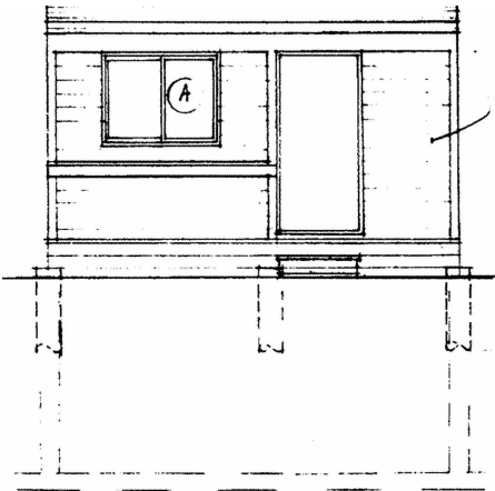
4 Entry Elevation
