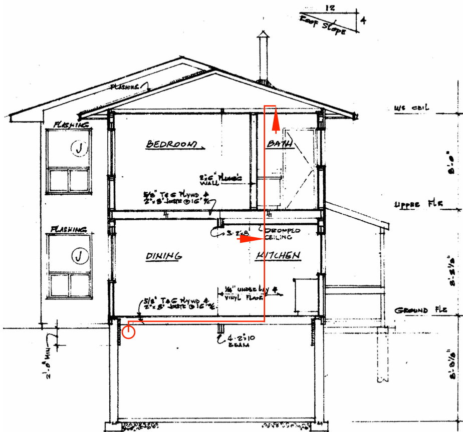
4/6 Section
