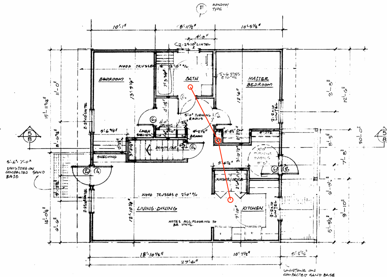
2/8 Ground Floor Plan
