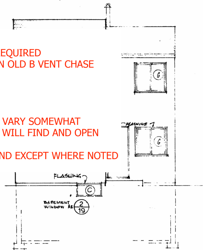
6/6 Patio Elevation
